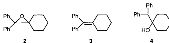
Scheme 1 SET = single electron transfer
